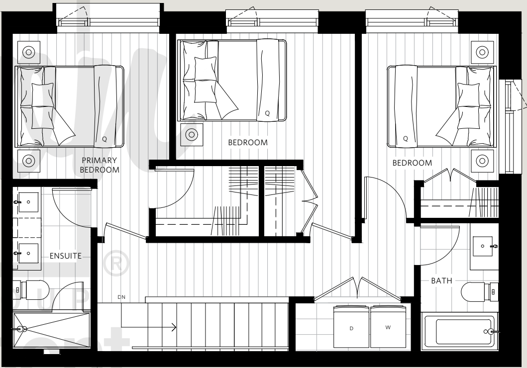
LEVEL 2
