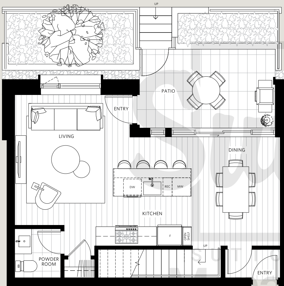
LEVEL 1
